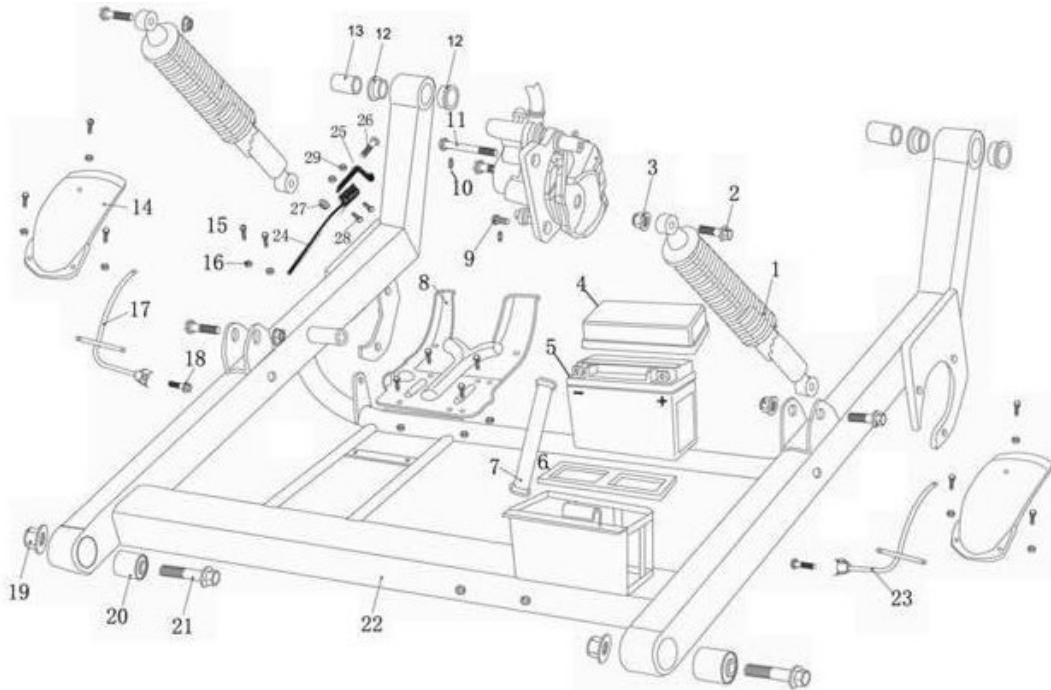
FIG.20 REAR SWING ARM
