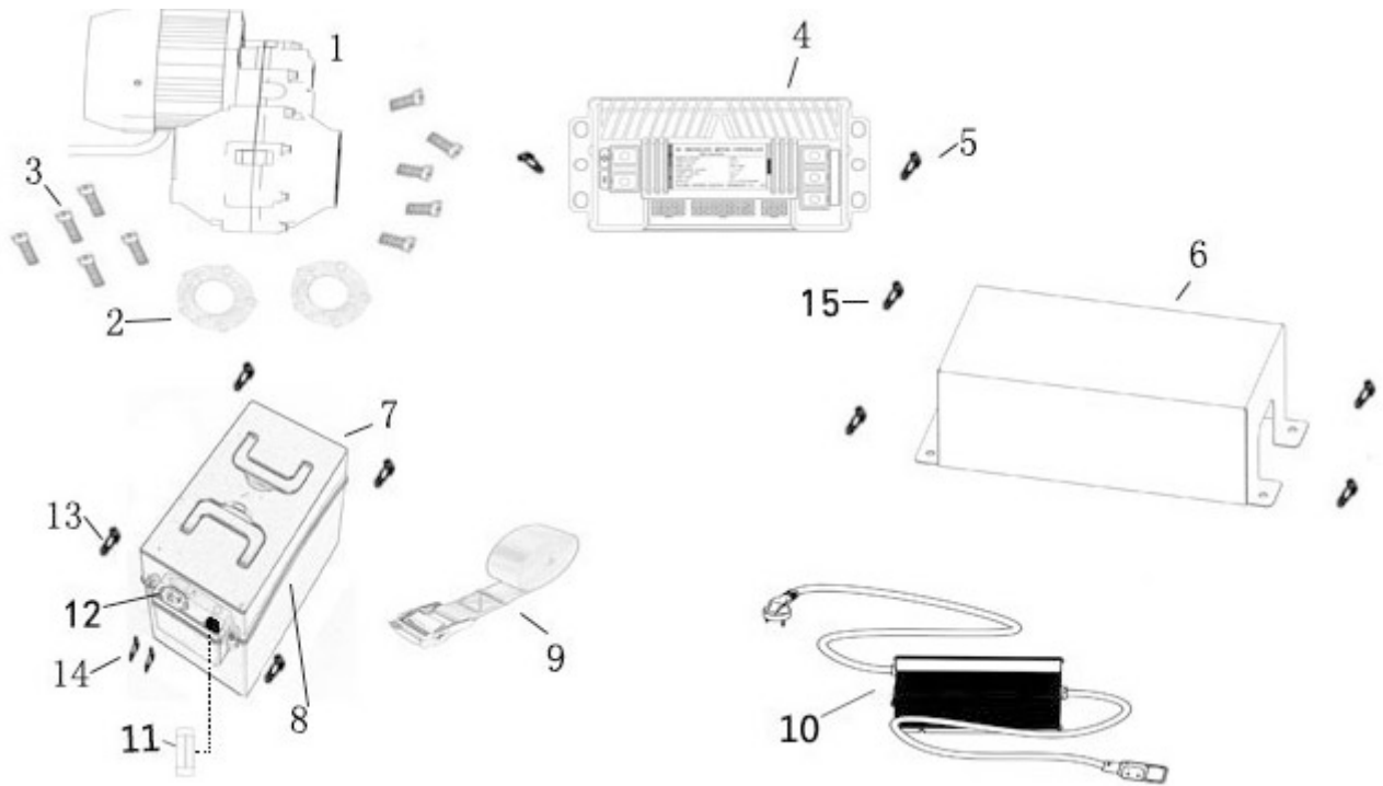
Fig 7: ELECTRIC MOTOR/CONTROLLER BATTERY ASSY
