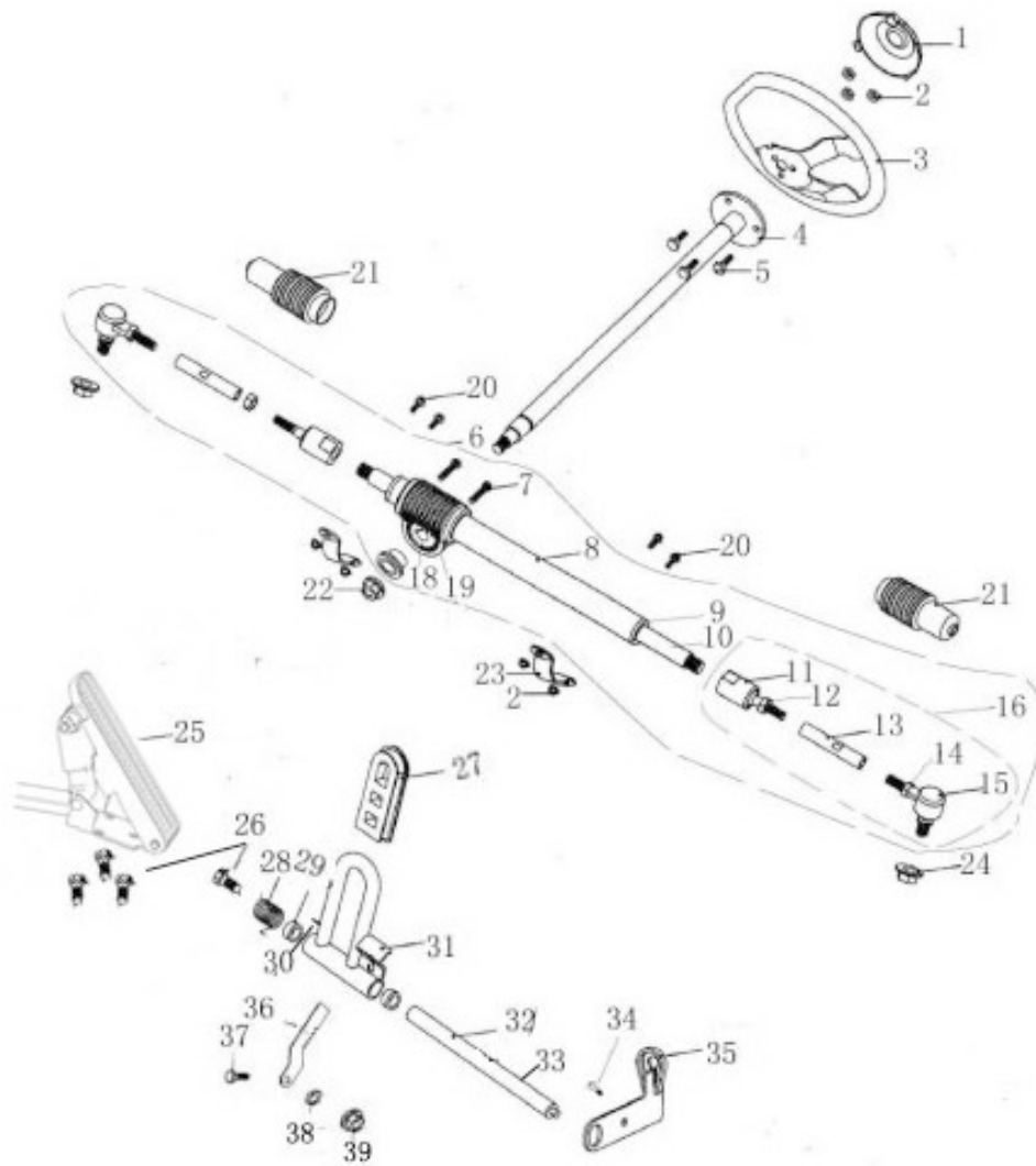
Fig 2: STEERING SHAFT ASSY
